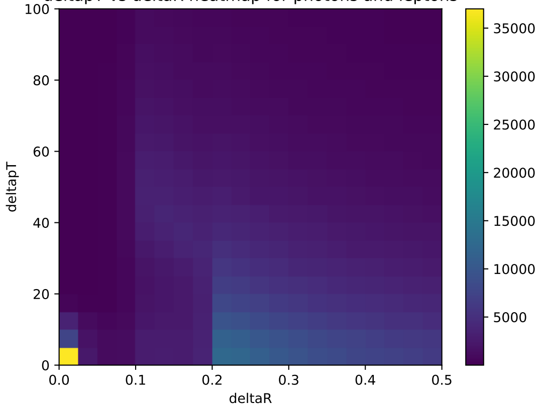
deltapT vs deltaR heatmap for photons and leptons
