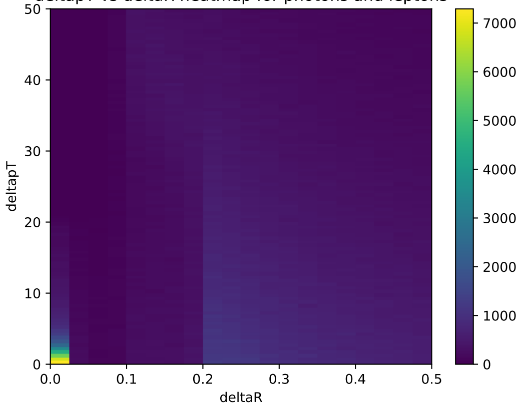
deltapT vs deltaR heatmap for photons and leptons
