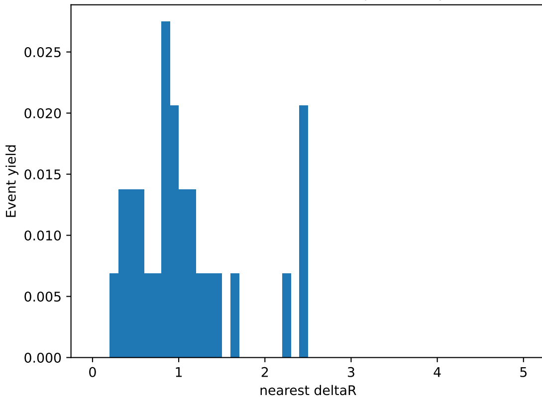
nearest deltaR between ph and lep
