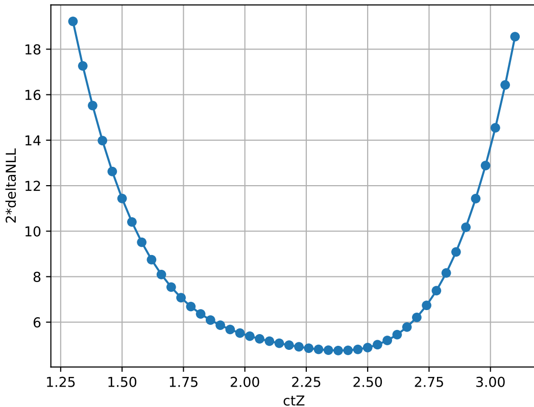
2 \cdot \text{deltaNLL} vs \text{ctZ} for \text{ctW} = 0.6600000262260437
