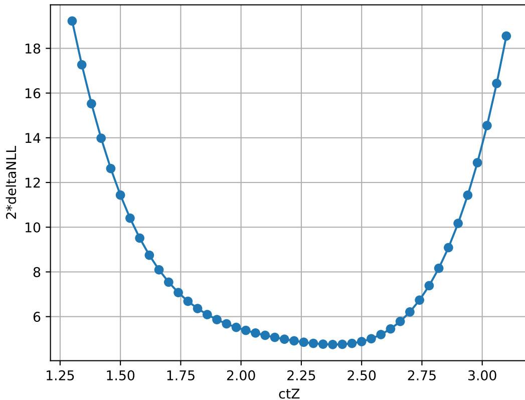
2 \cdot \text{deltaNLL} vs \text{ctZ} for \text{ctW} = 1.8200000524520874
