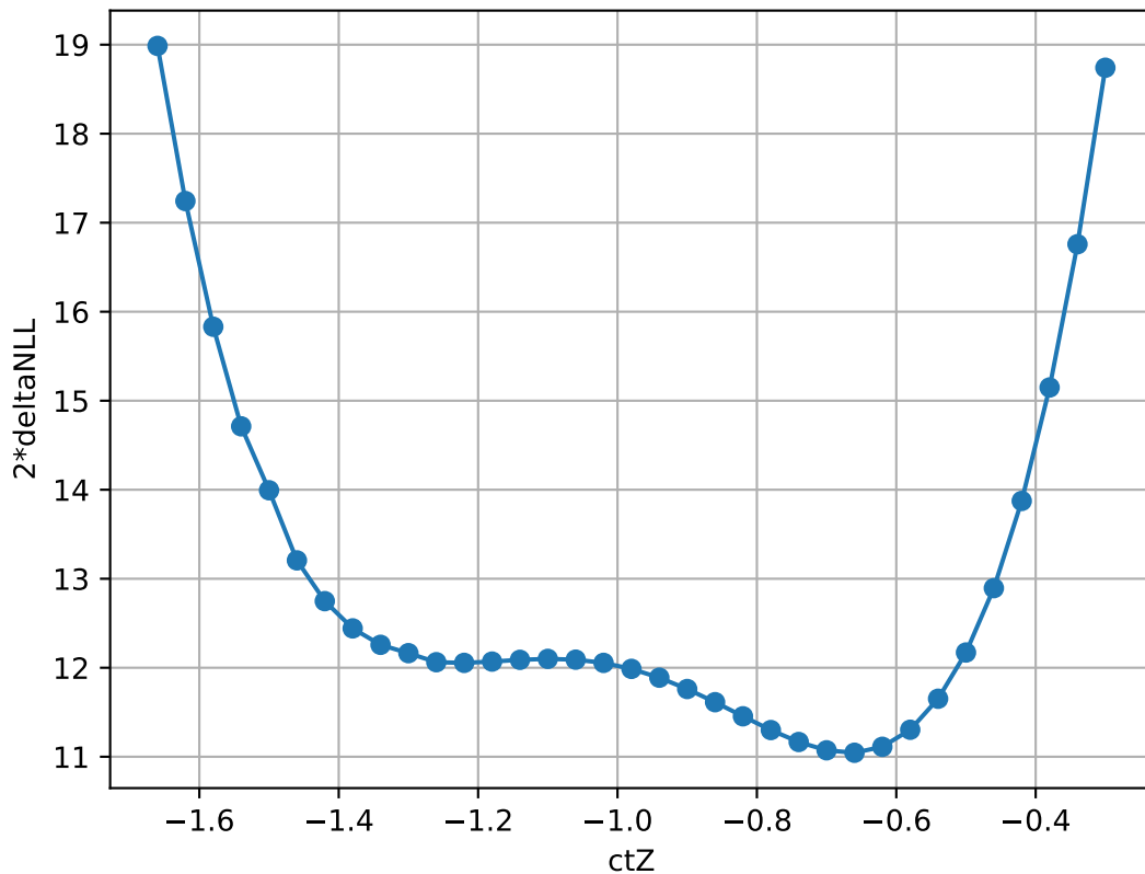
2 \cdot \text{deltaNLL} vs \text{ctZ} for \text{ctW} = -0.9399999976158142
