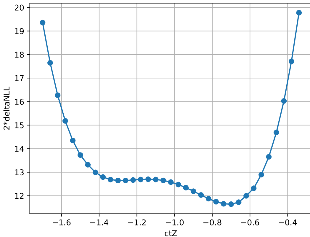
2*deltaNLL vs ctZ for ctW = -0.9800000190734863
