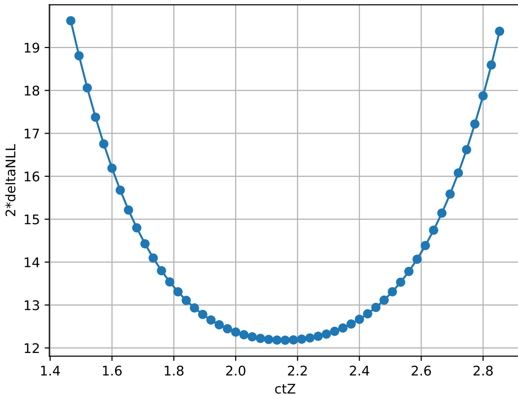
2*deltaNLL vs ctZ for ctW = 1.8133333921432495
