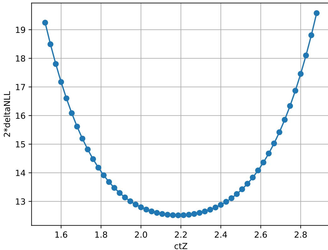
2 \cdot \text{deltaNLL} vs \text{ctZ} for \text{ctW} = 1.840000033378601
