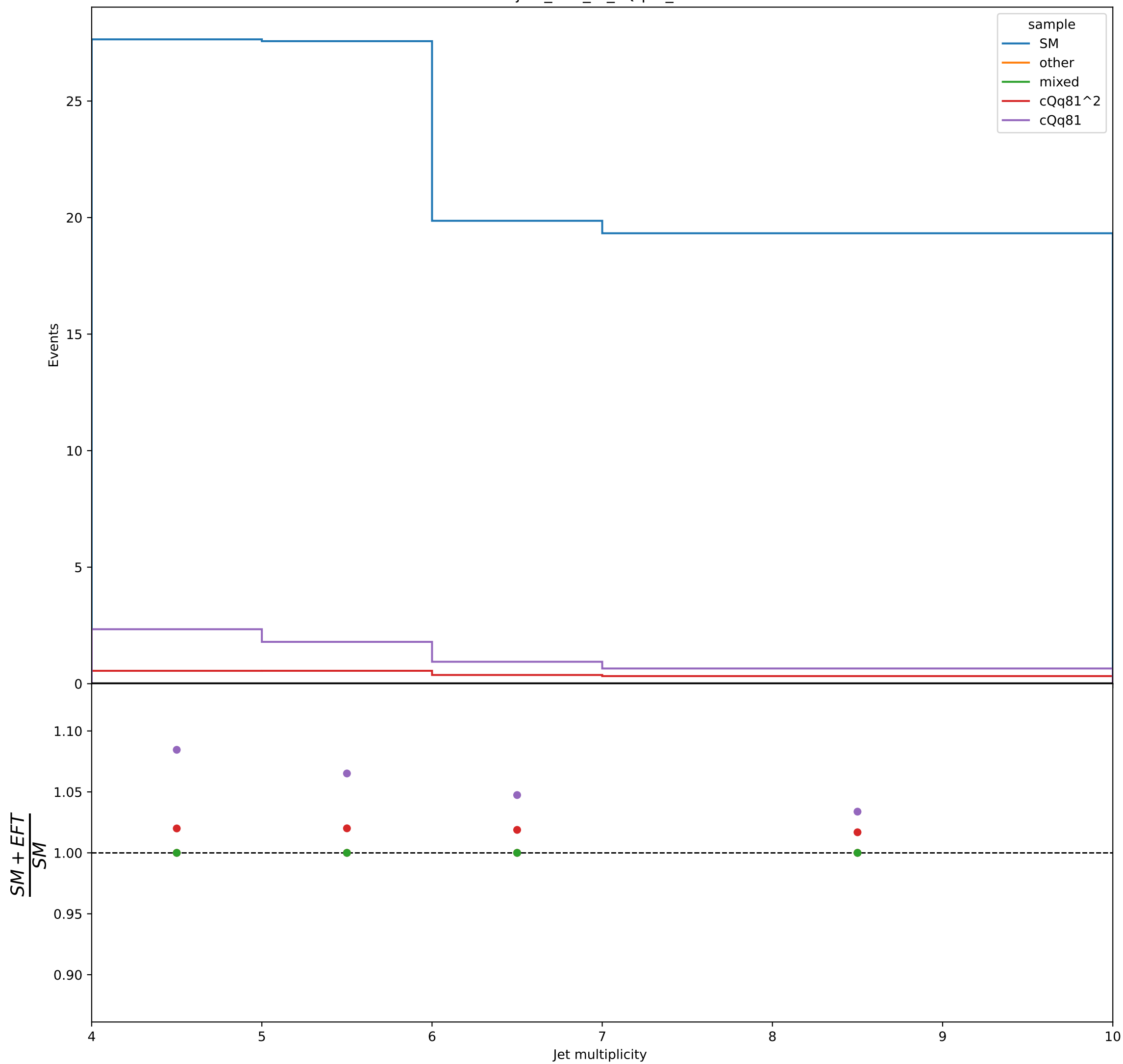
njets_2lss_4t_cQq81_0.5
