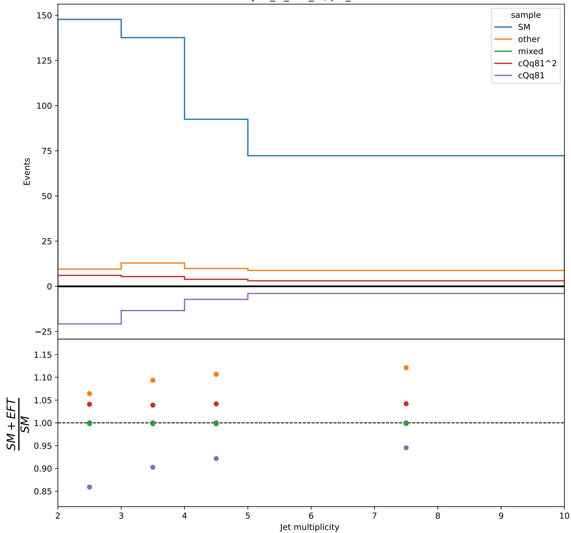
njets_3l_offZ_cQq81_-0.85
