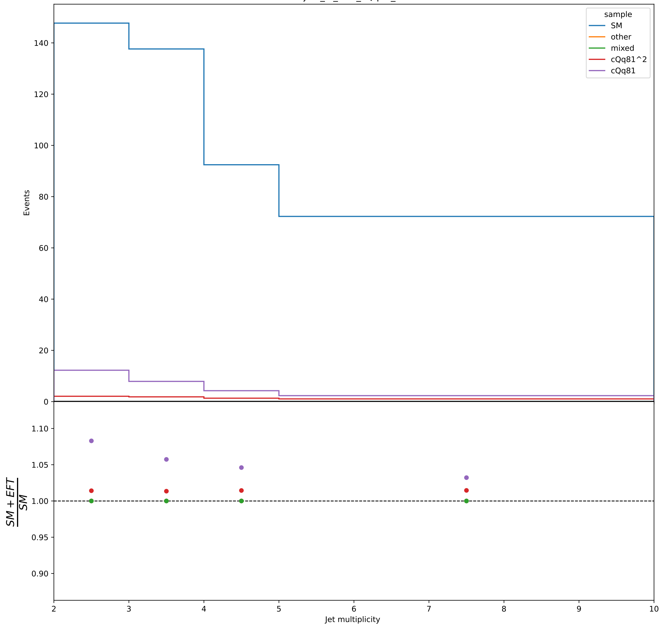
njets_3l_offZ_cQq81_0.5
