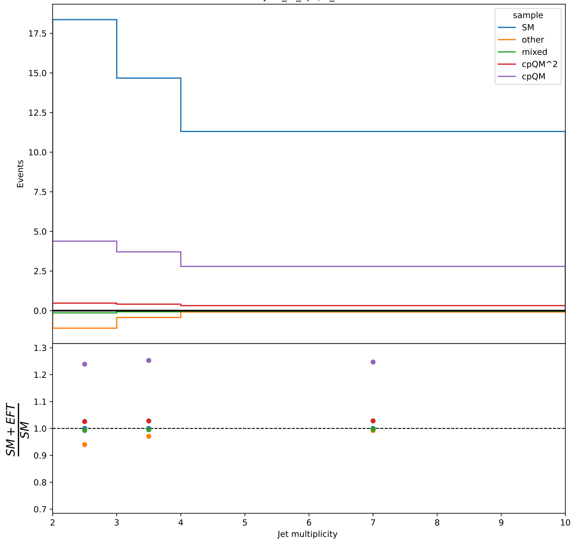
njets_4l_cpQM_-2.72
