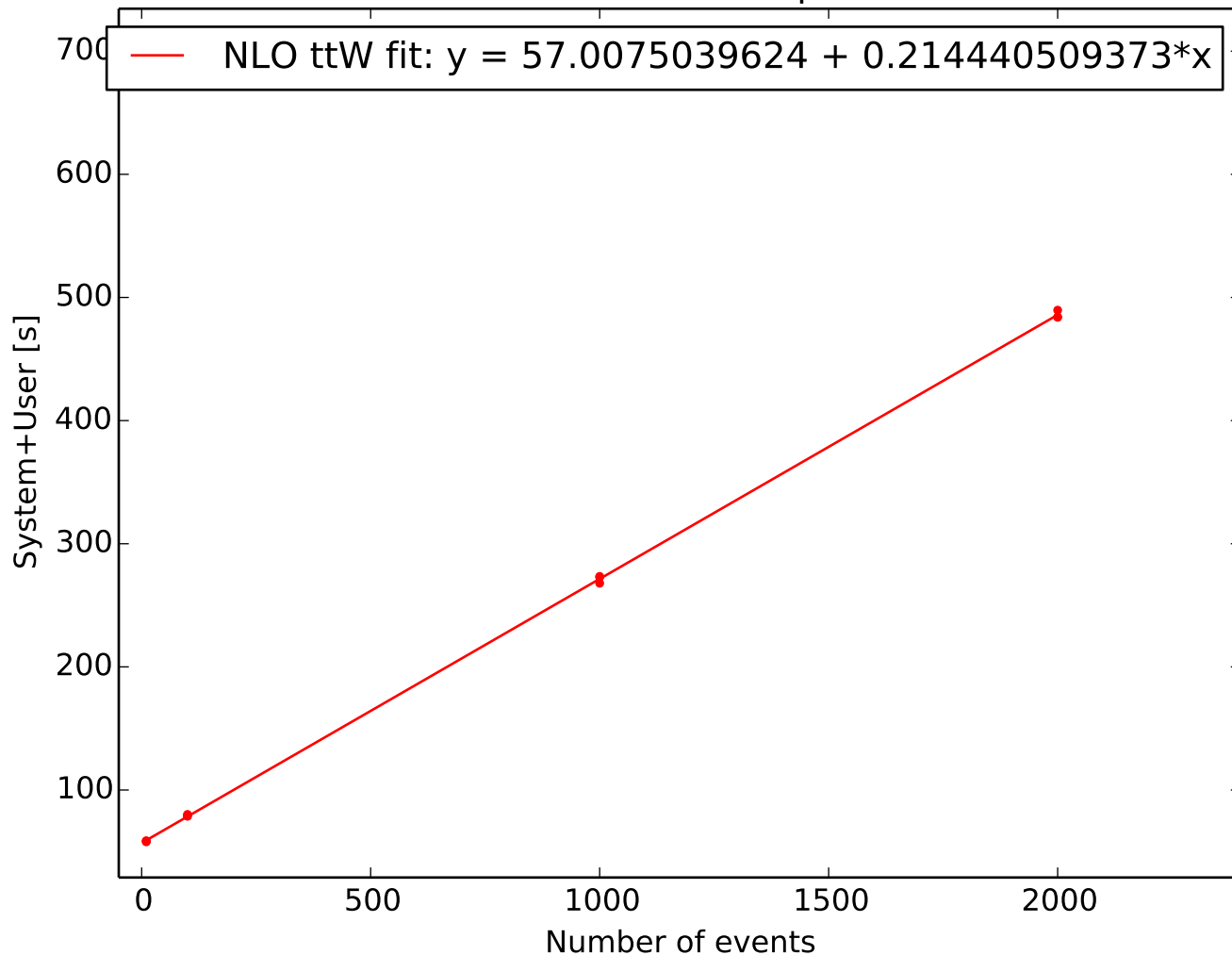
LO vs NLO CPU comparison
