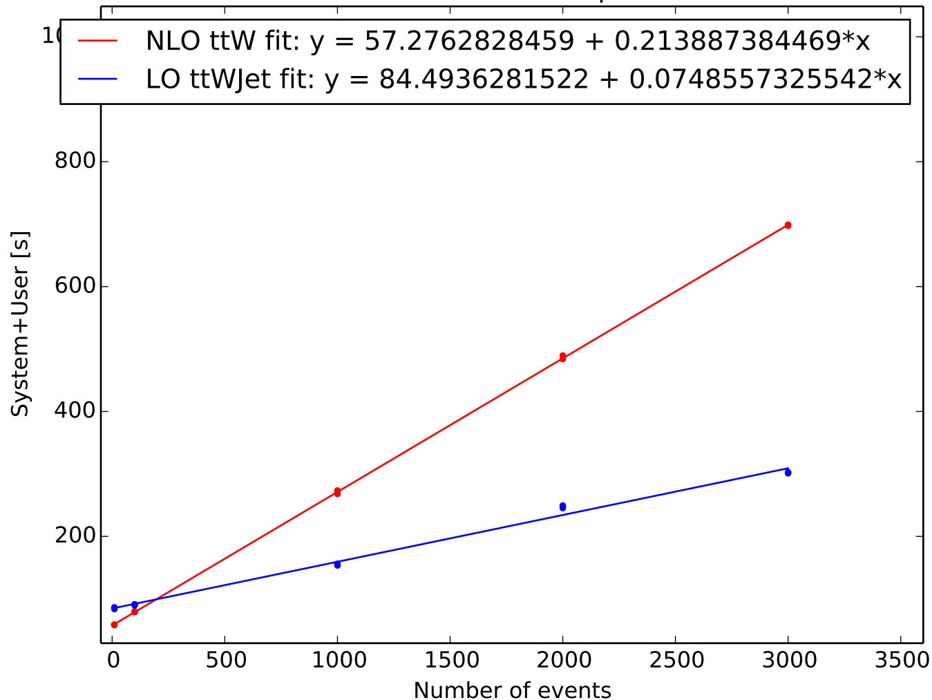
LO vs NLO CPU comparison
