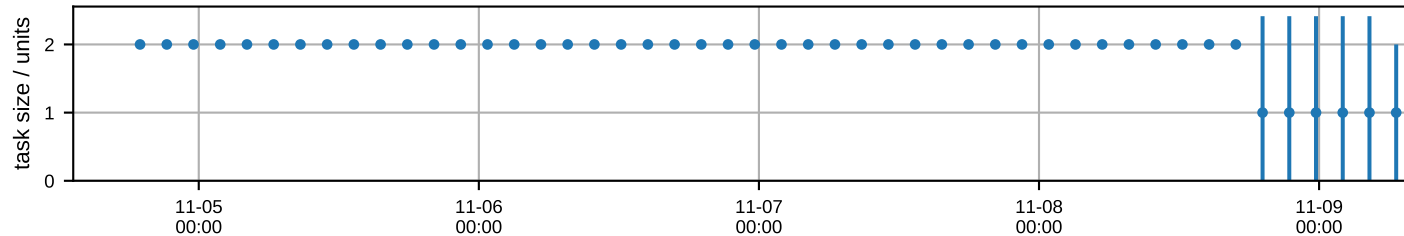
reco_step_tllq4fNoSchanWNoHiggs0p_HanV4Model16DtllScanpointsXQCUT0MatchOff_run1
